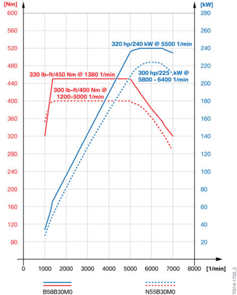
Performance diagram of the B58B30M0 engine
