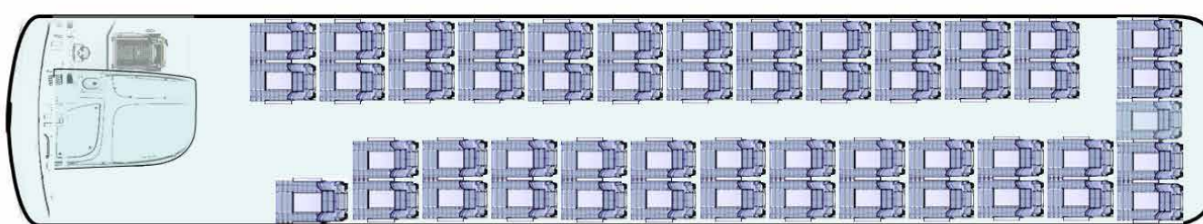
TF25 13.5 G6R - 52 + D (2x2) Push back seat with FOH door
